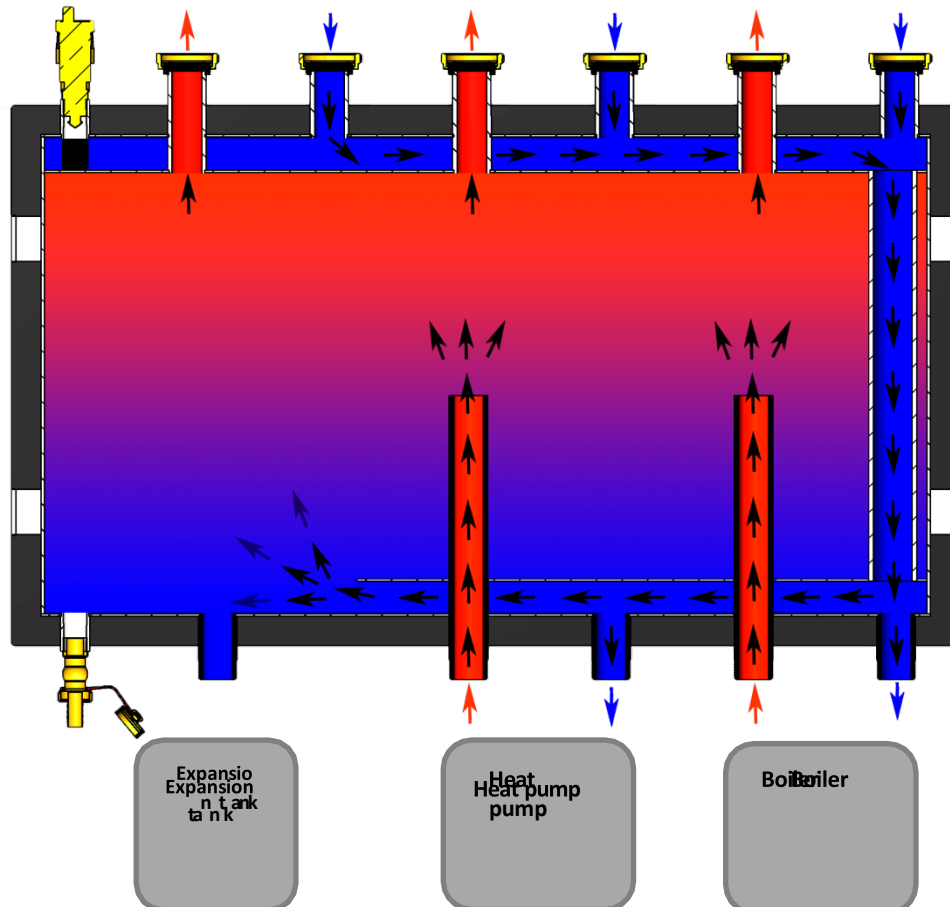
Flow diagram of the coolant in the Uni-Tank
