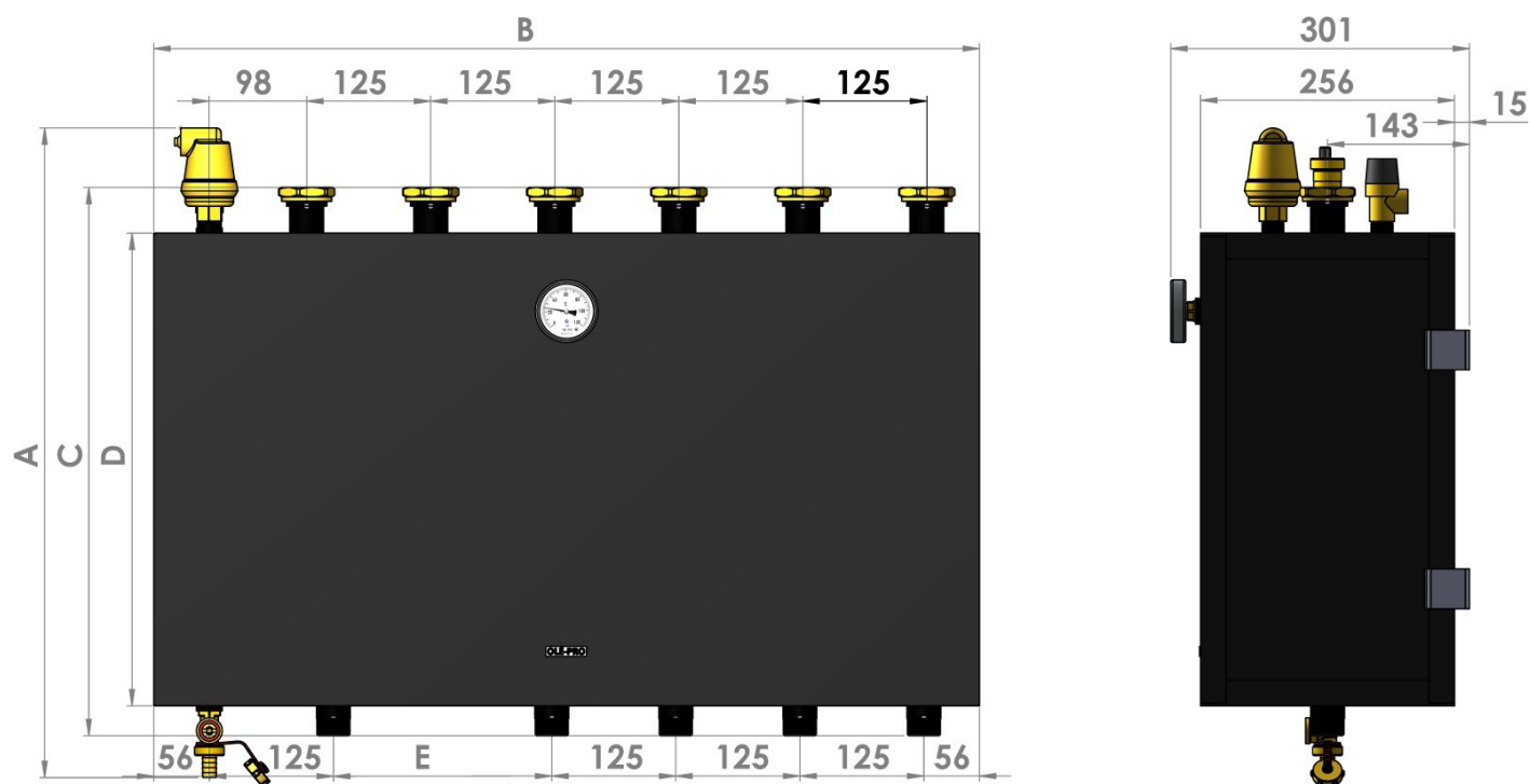
Overall and connecting dimensions
