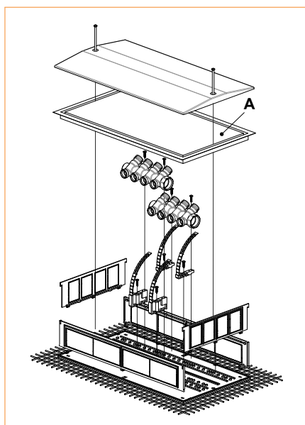
(c) Modular manifold CI 300NB/NR installation.
